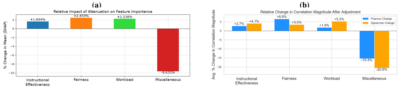
Figure 5. Mechanistic coherence checks after attenuation. (a) Relative changes in SHAP-based feature importance, computed on held-out professors ( n = 3,414 reviews). (b) Average relative change in correlation magnitude (Pearson and Spearman) after adjustment, held-out professors ( n = 2,052 ). Bars show mean (|corr_{adjusted}| - |corr_{raw}|) / |corr_{raw}| across polarity groups.
